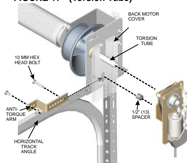
FIGURE 17 (Torsion Tube)
