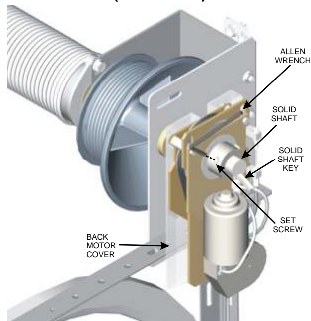
FIGURE 18 (Solid Shaft)
