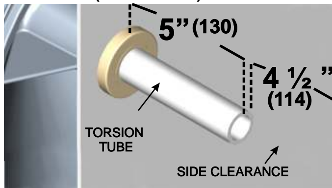
FIGURE 13 (Torsion Tube)
